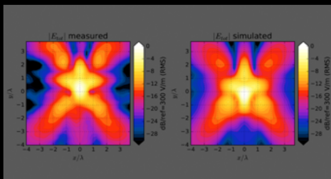
Measured E-field (left) compared to the simulations (right) at 30 GHz.
