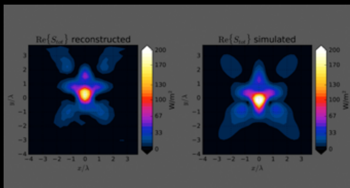
Reconstructed power density (left) from measurements compared to simulation (right).
