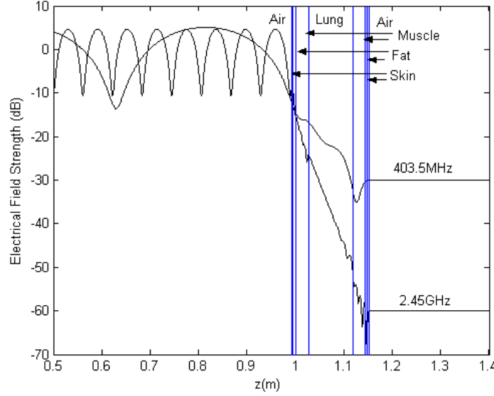
Figure 4.6: Electric field strength dependence on frequency.
